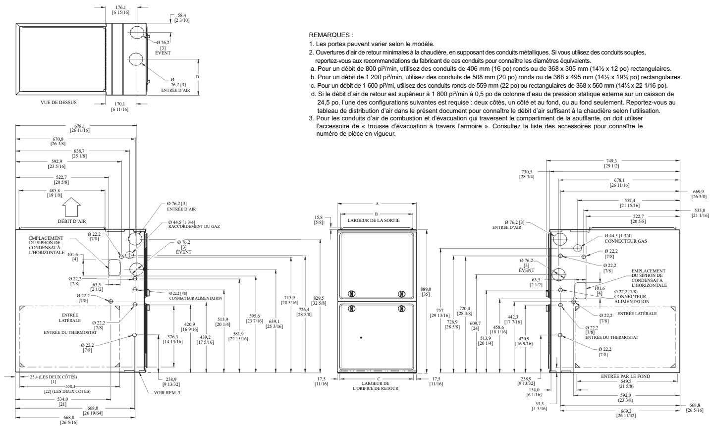
Figure 1 – Plan dimensionnel
