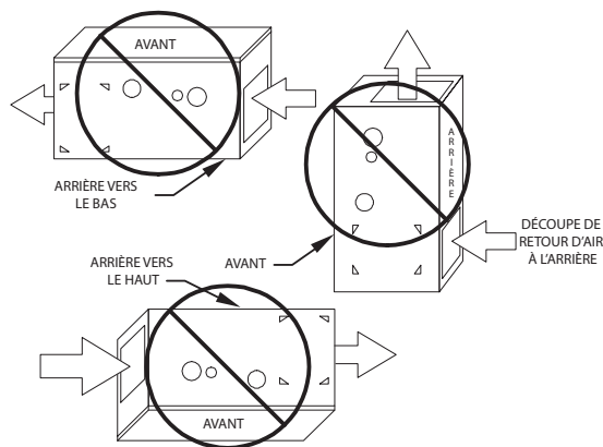
Figure 4 – Installations interdites
