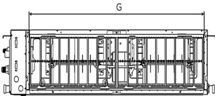
Air inlet dimensions
