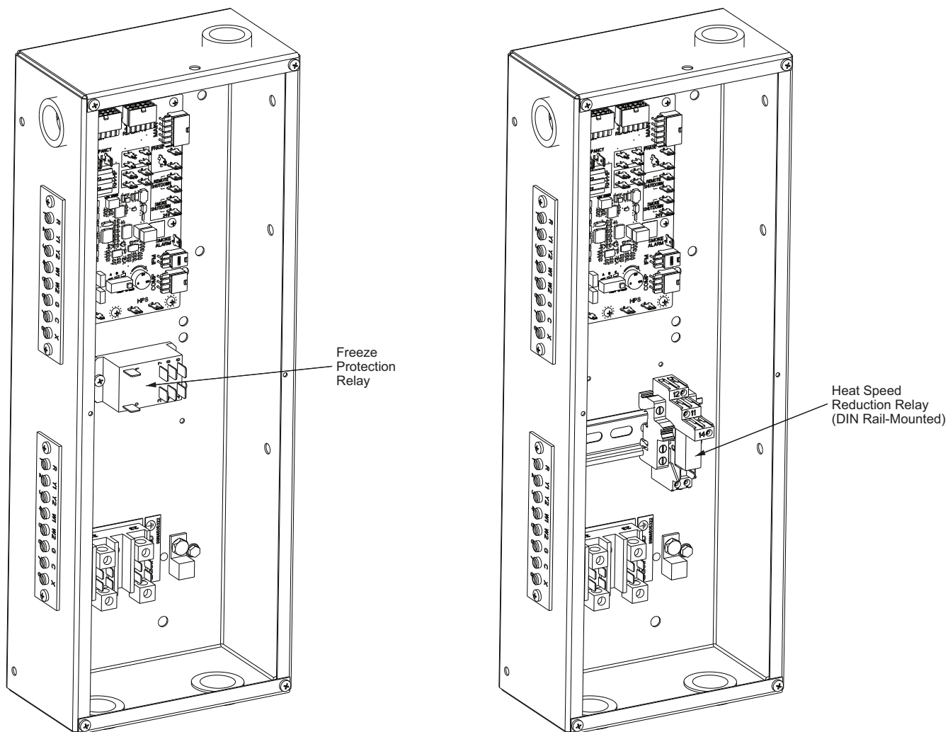
Fig. 17 — Unit Control Box with Freeze Protection Relay
