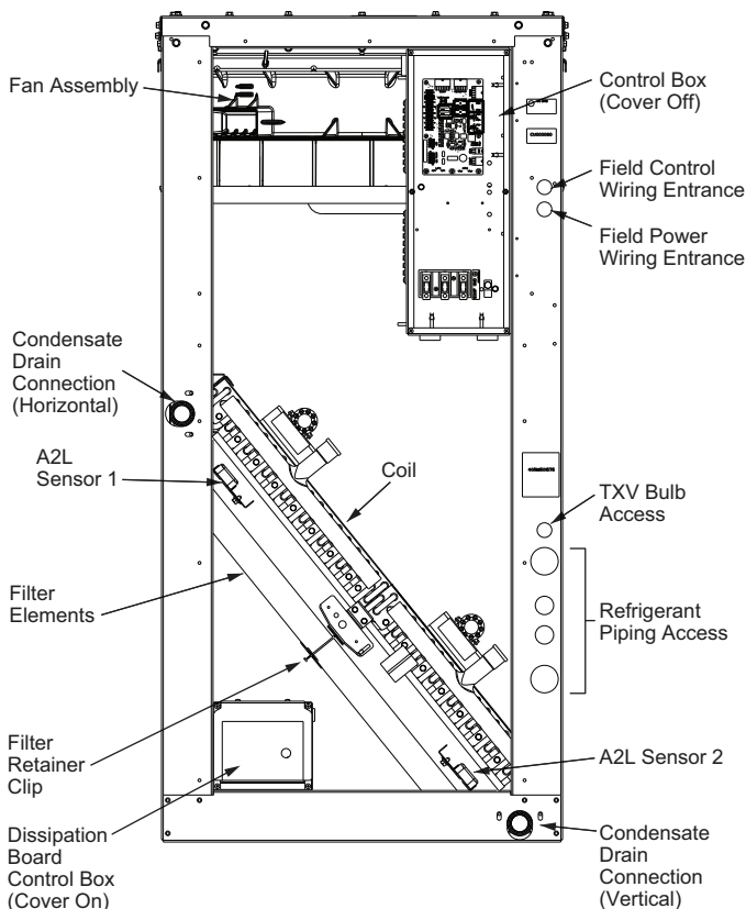
Fig. 15 — Wiring and Service Access (Side Panel Removed)
