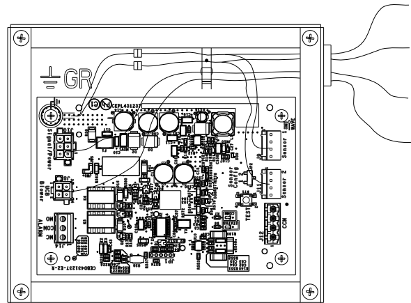
Fig. 25 — Dissipation Control Box
