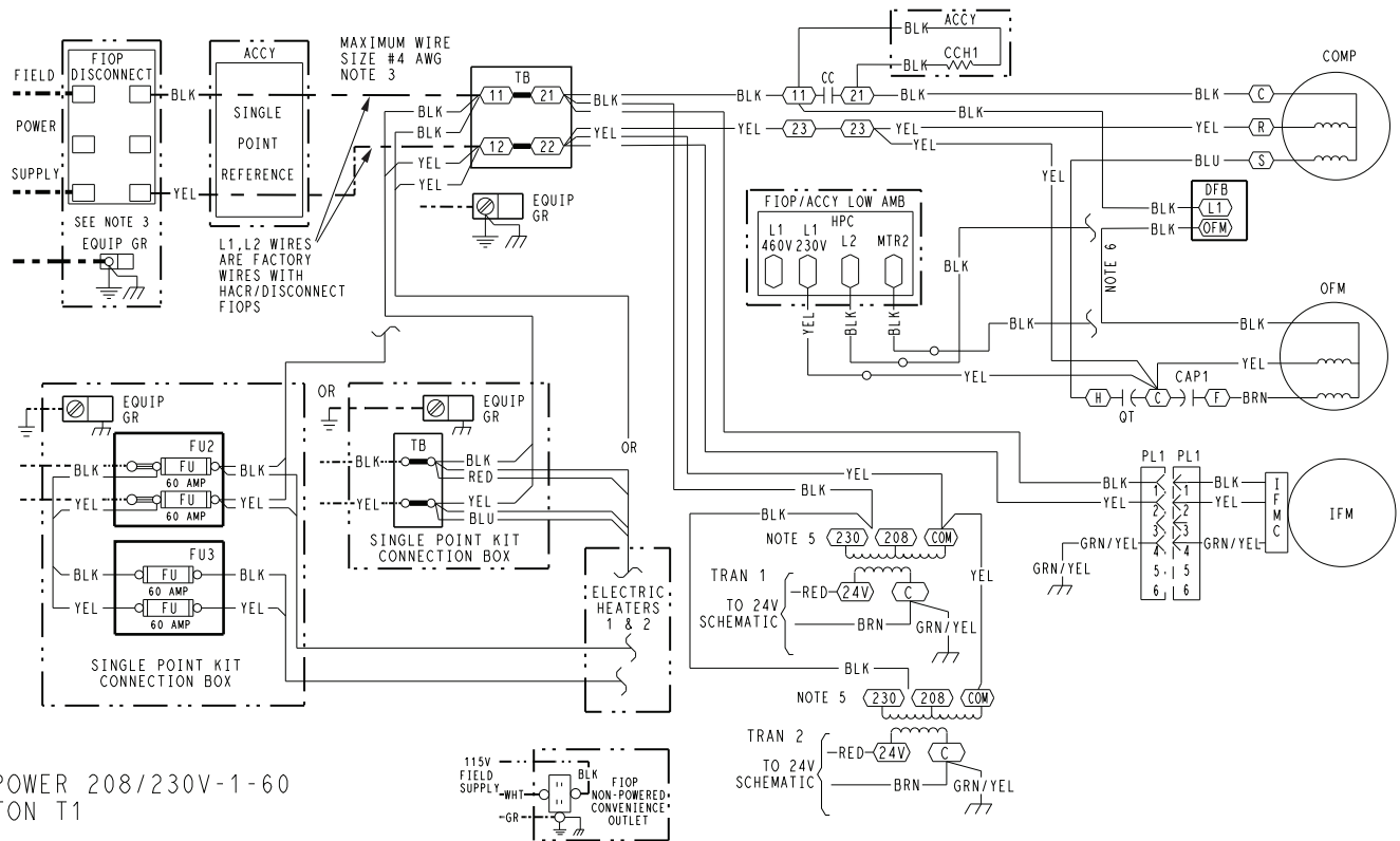
Typical 50FCQA04-06 Power Wiring Diagram, 208-230/1/60 Unit
