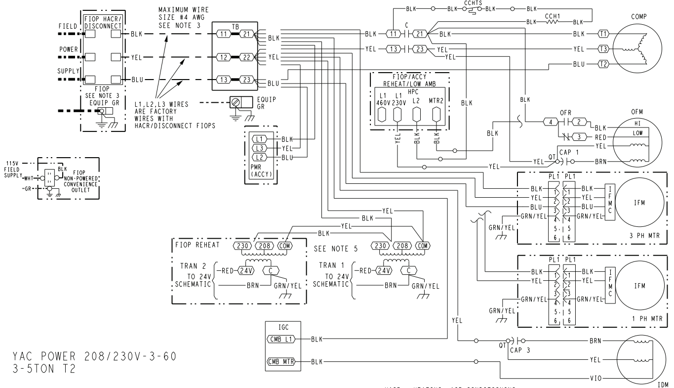
TYPICAL 48GC 04-06 POWER WIRING DIAGRAM, 208-230/3/60 UNIT SHOWN
