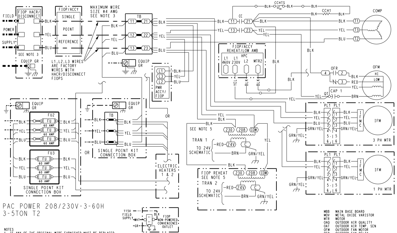
TYPICAL 50GC 04-06 POWER WIRING DIAGRAM, 208-230/3/60 UNIT SHOWN
