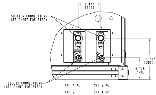
DETAIL A (NOTE POSITION OF CKT 1)
