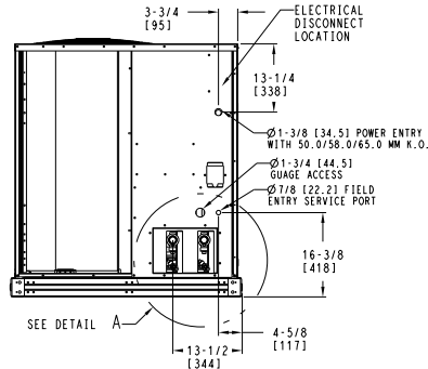
LEFT SIDE VIEW (FOR 38AXD/38AXQ SYSTEMS)
