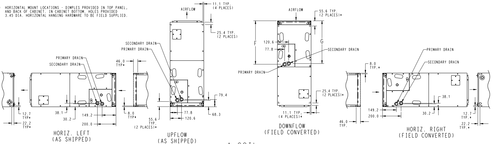
Fig. 4 – Dimensions, sheet 4
