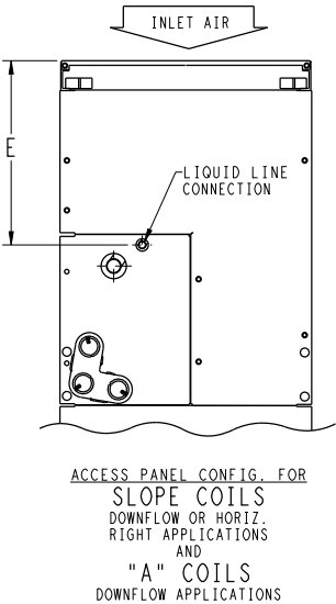
Fig. 3 – Dimensions, sheet 3
