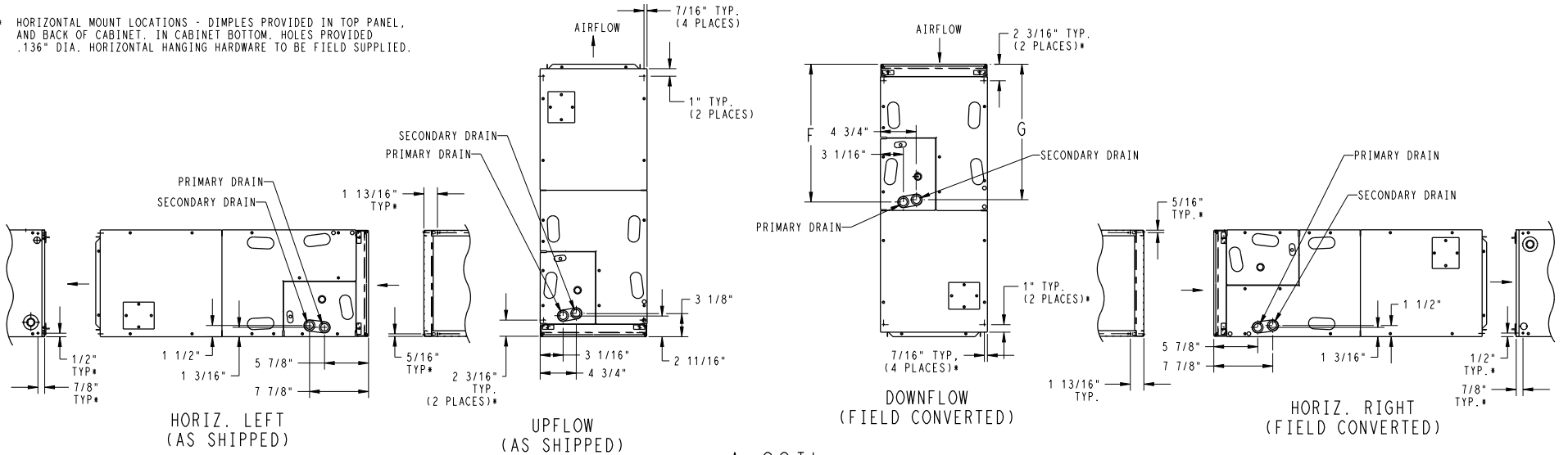
Fig. 2 – Dimensions, sheet 2
