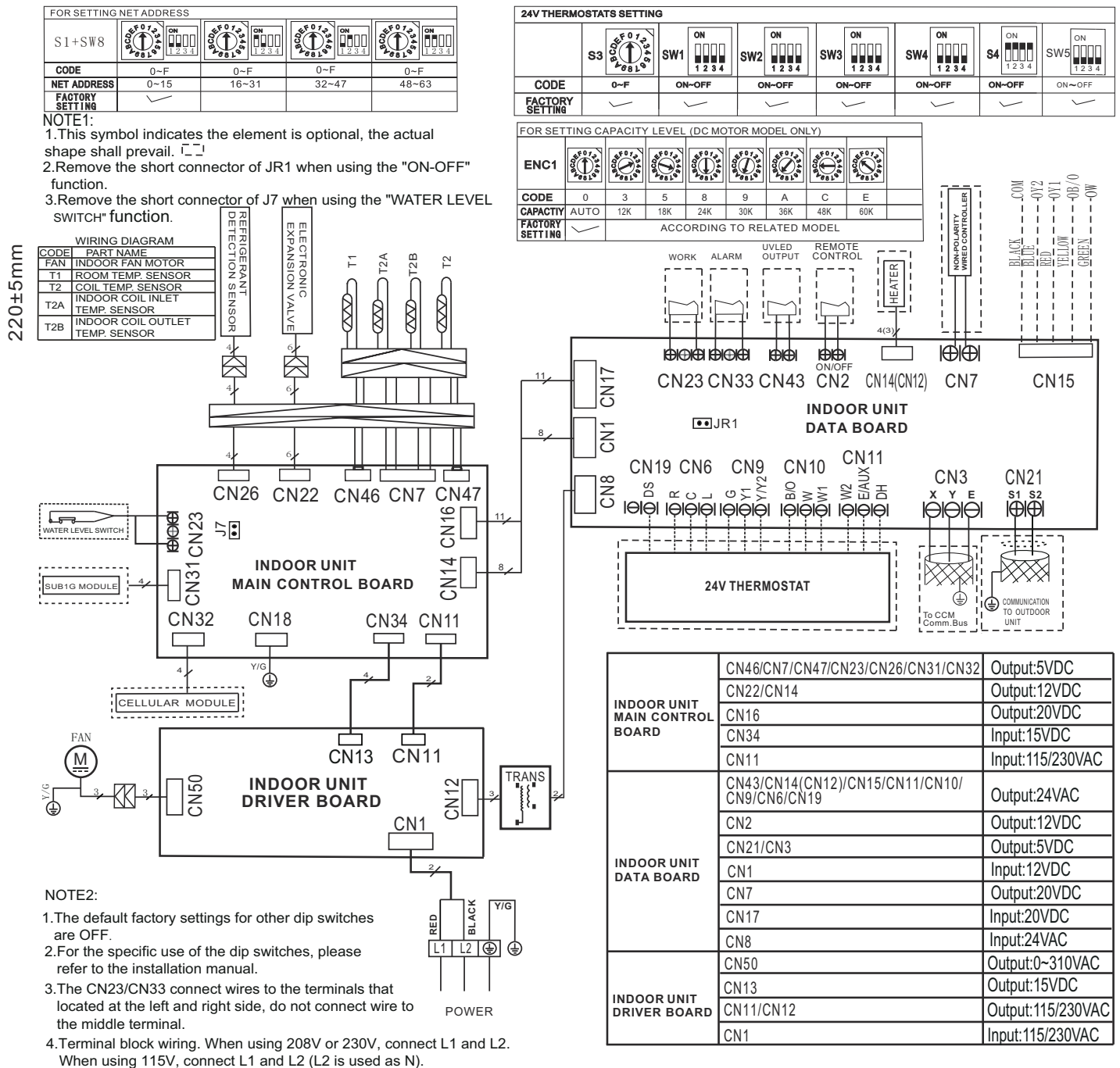
Fig. 22 — Wiring Diagram (For All Sizes)
