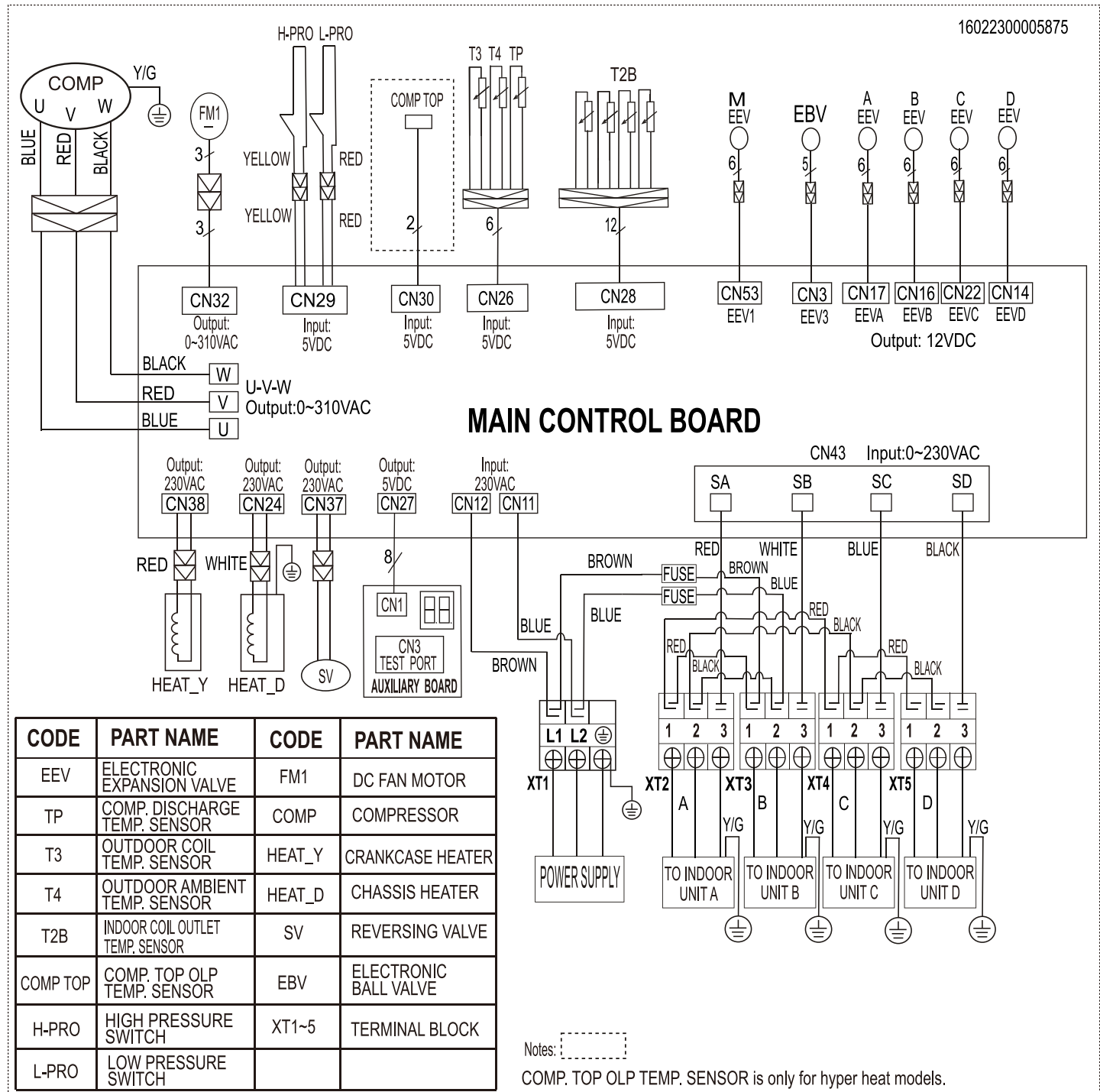
Fig. 15 — Wiring Diagram 24K
