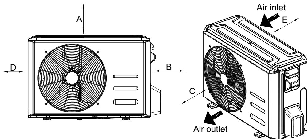
Fig. 7 — Clearances
