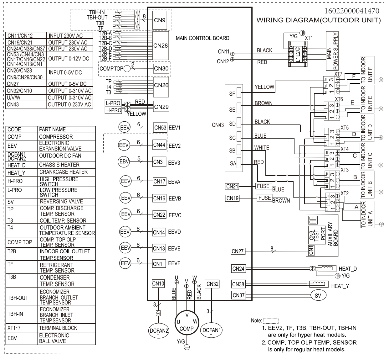
Fig. 17 — Wiring Diagram 48K/55K
