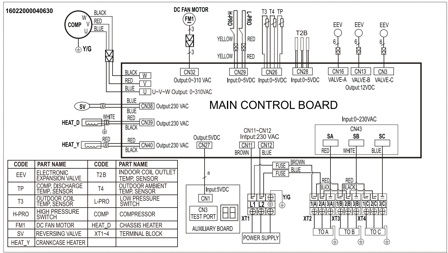
Fig. 14 — Wiring Diagram 18K
