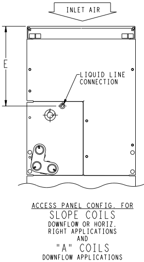
Fig. 3 – FJ5 - Metric (sheet 1)
