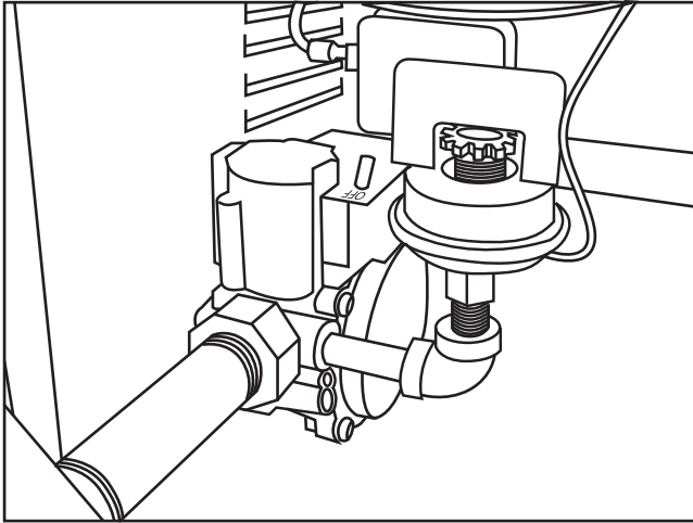
Fig. 4 — LP Pressure Switch Piping (36G Gas Valve Shown)
