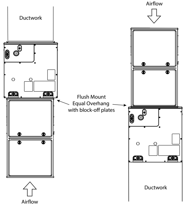
Fig. 4 – Smaller Furnace, Equal Overhang, Flush Mount (not recommended) A221123A
