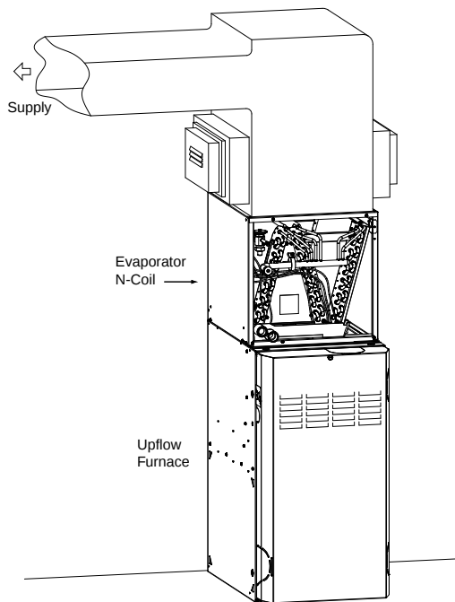
Fig. 10 – Humidifier Application
