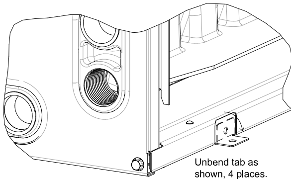
Fig. 8 – Horizontal-Left Installation A13064
