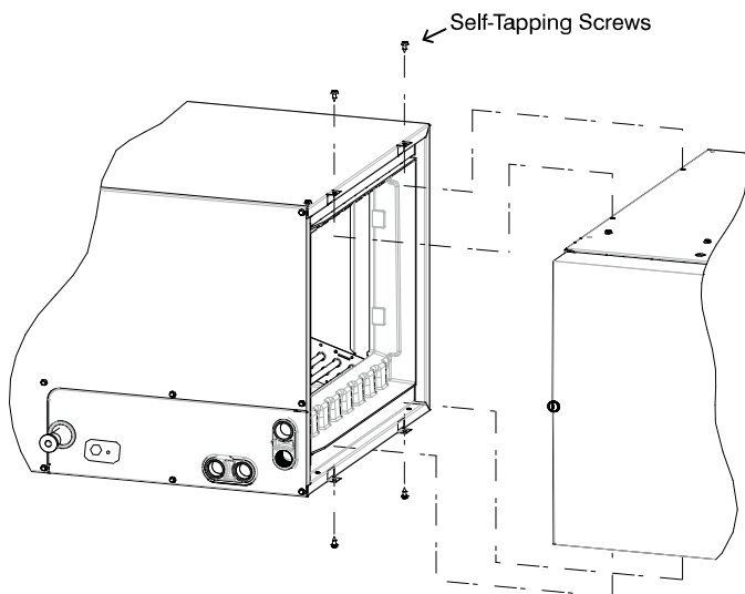
Fig. 9 – Horizontal-Left Installation A13066A
