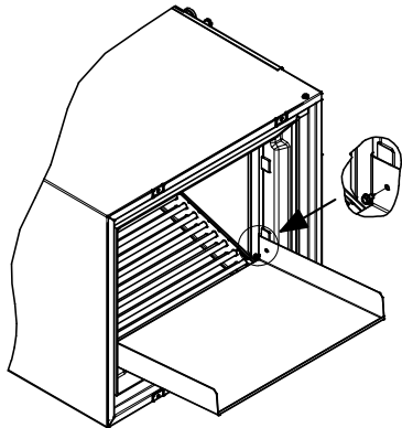
Fig. 7 – Condensate Pan Extension Cork Tape Location A170282A
