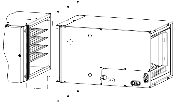
Fig. 6 – Horizontal-Right Installation
