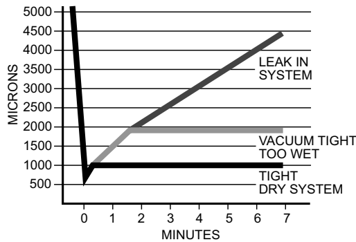
Fig. 10 – Deep Vacuum Graph
